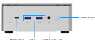
Front I/O
