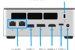
Rear I/O
